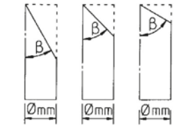
Max Ø mm x β° 37x30° 52x45° 64x60°
