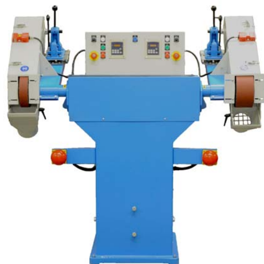
Powerfin Bull , double-ended belt grinder, with customised knee control and guarding
