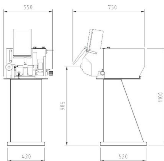
Powerfin 1060, mounted on a pedestal
